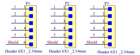
Din5-F-BO-V1A Schematic Diagram
